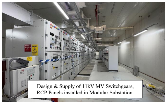
MV Panels
