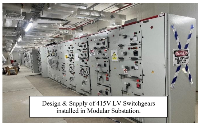
LV Panels
