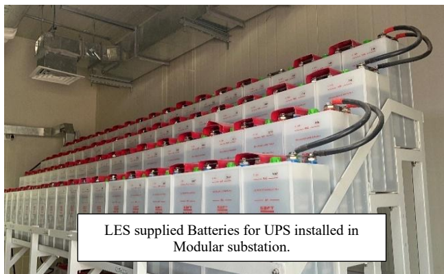
Battery Room
